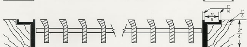
Drop in Grille Using Type D Frame
