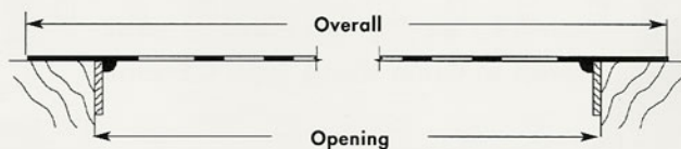
Grille set in top surface with inner frame to prevent movement
