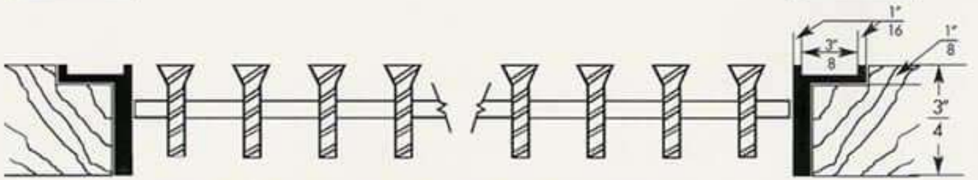
Wide Drop in Grille Using Type D Frame
