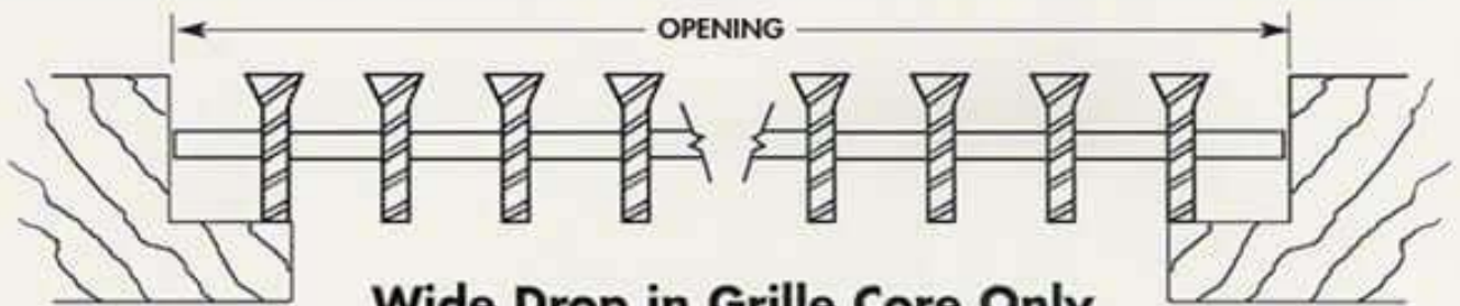
Wide Drop in Grille Core Only
