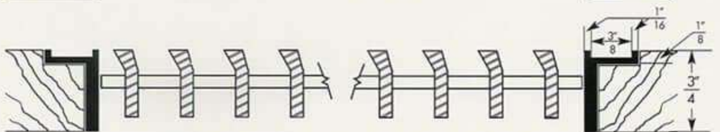
Drop in Grille Using Type D Frame
