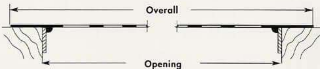
Grille set in top surface with inner frame to prevent movement
