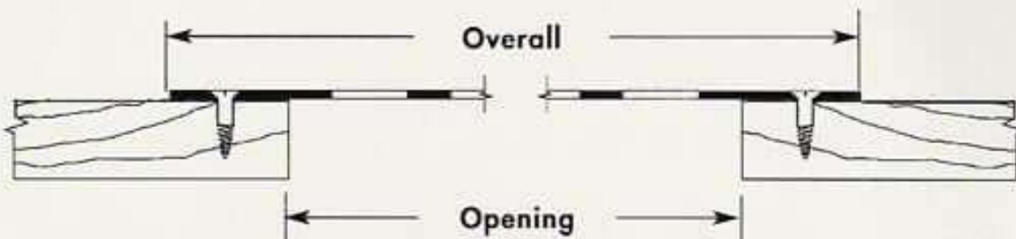
Grille on top of frame with countersink holes
