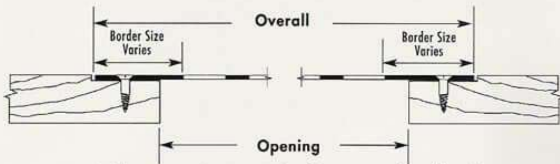
Grille connection mortised into woodwork with countersink holes for flush mounting
