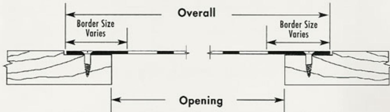
Grille connection mortised into woodwork with countersink holes for flush mounting
