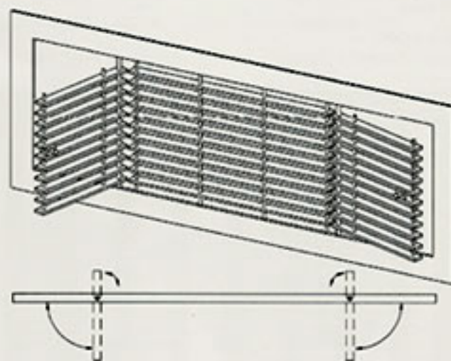
BAR GRILLE WITH ACCESS DOORS
